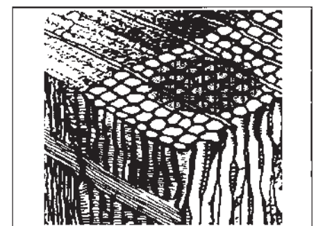
High pressure injection can damage the thin cell walls in the sapwood
